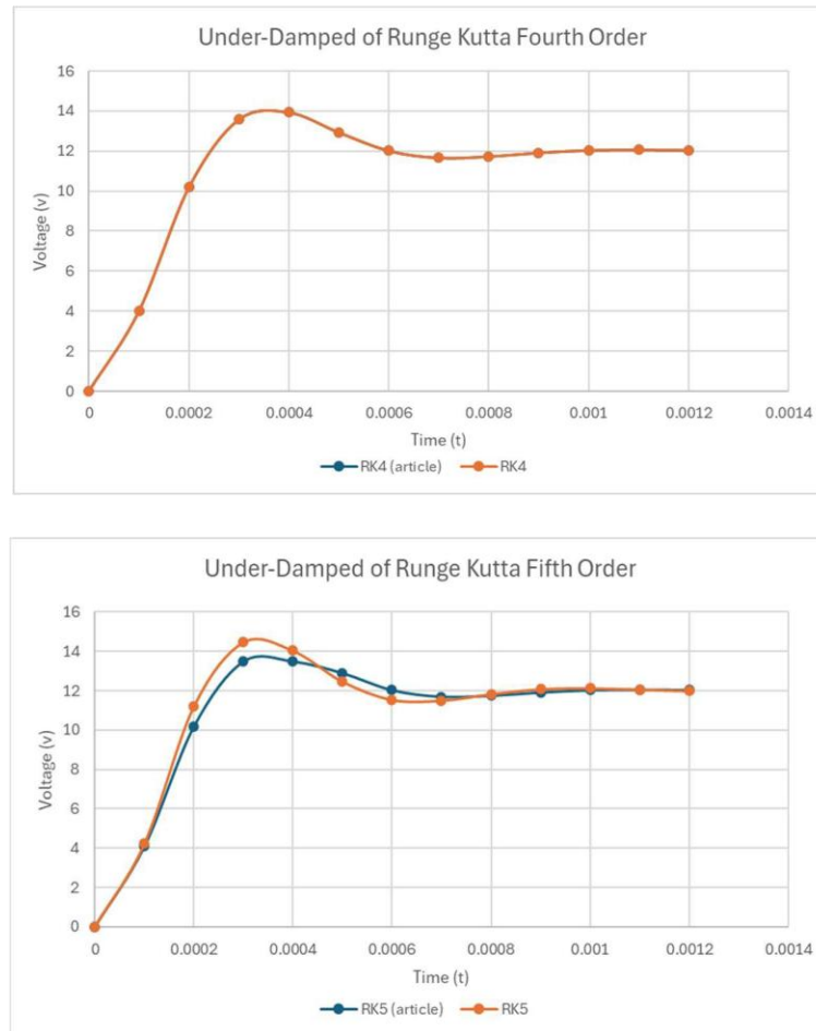
Figure 1: Voltage-Time Response of the Underdamped RLC Series Circuit
